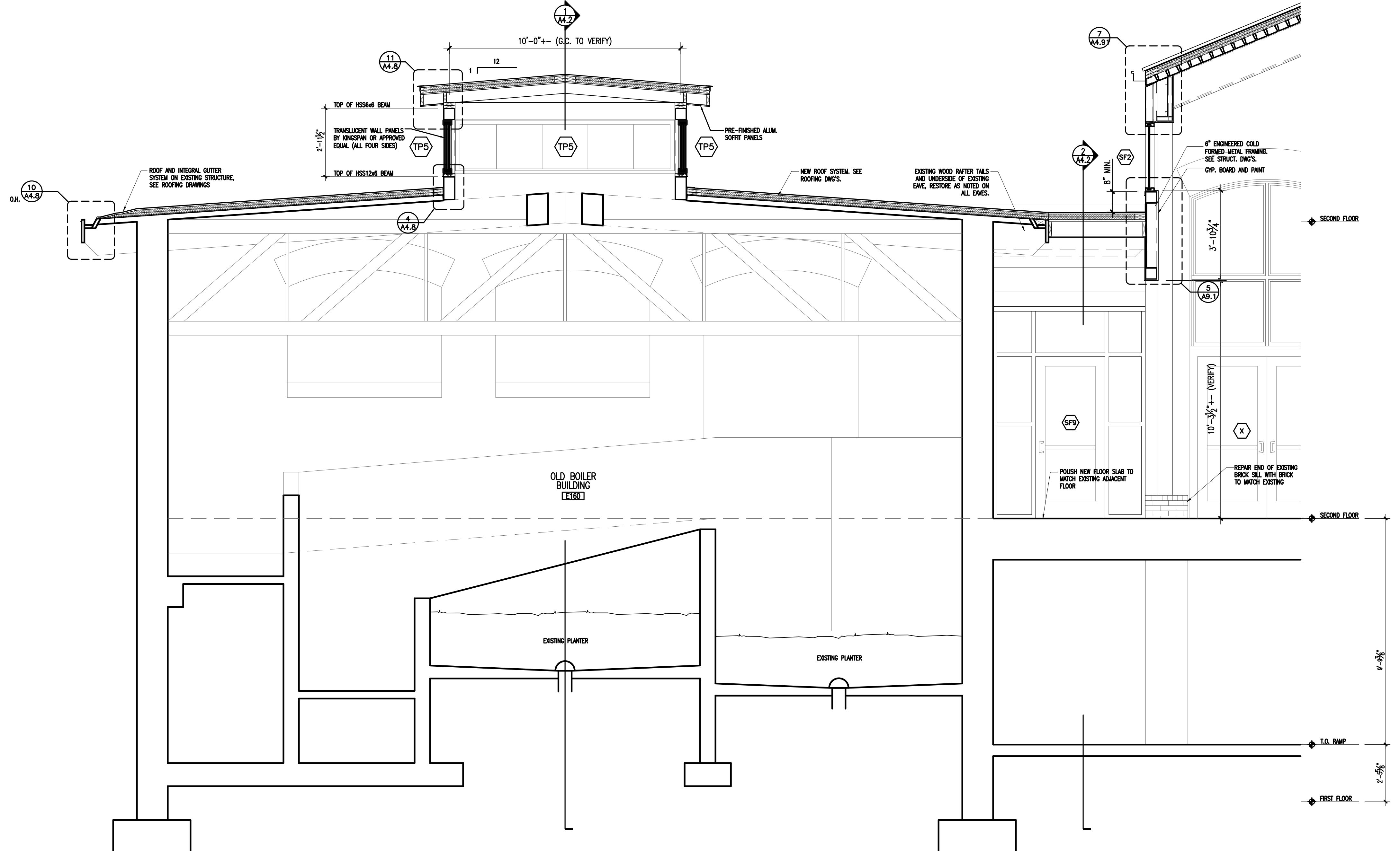
2 SECTION THRU OLD BOILER HOUSE/CONNECTOR SCALE: 3/8" = 1'-0"
