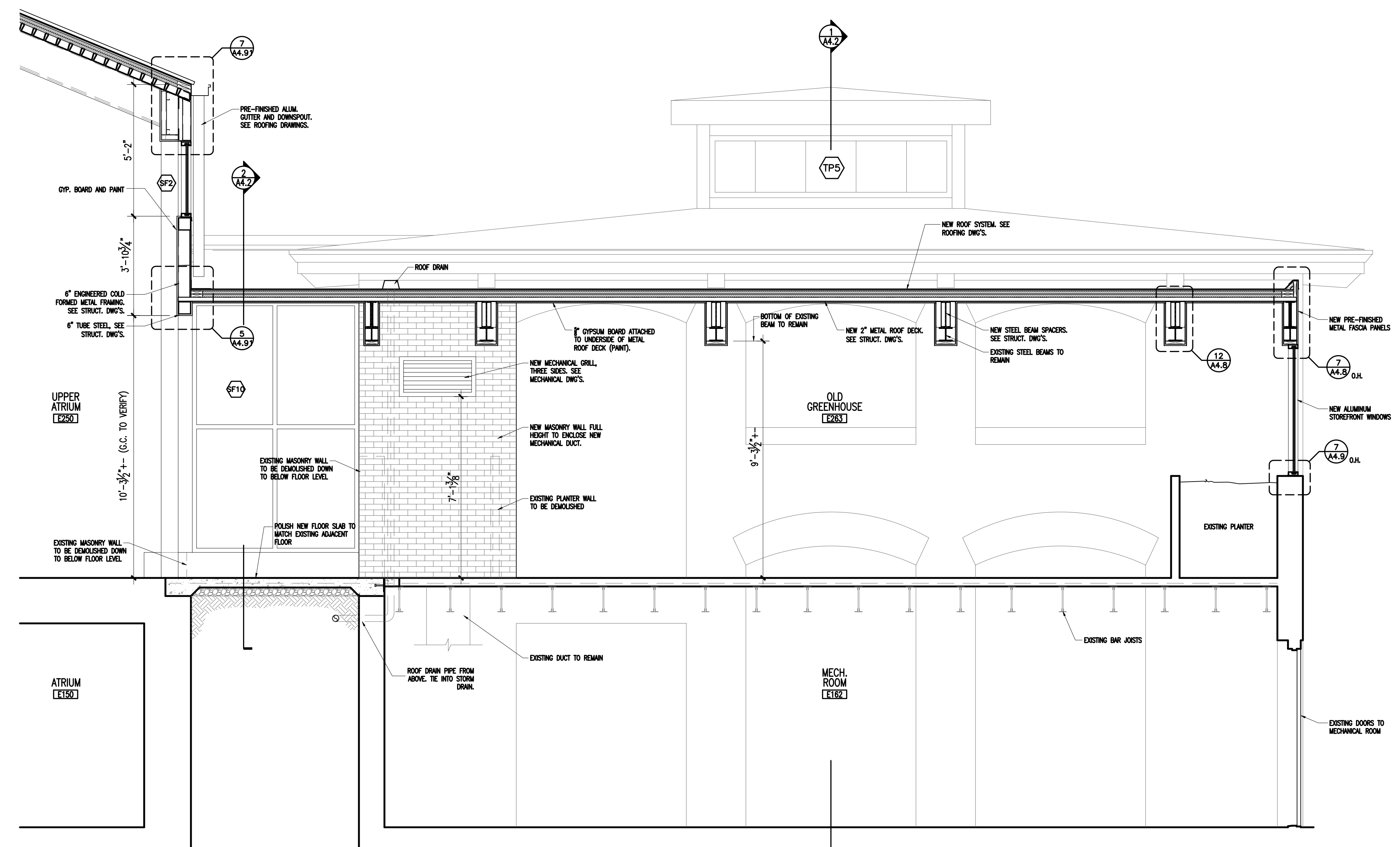
1 SECTION THRU GREENHOUSE/CONNECTOR SCALE: 3/8" = 1'-0"
