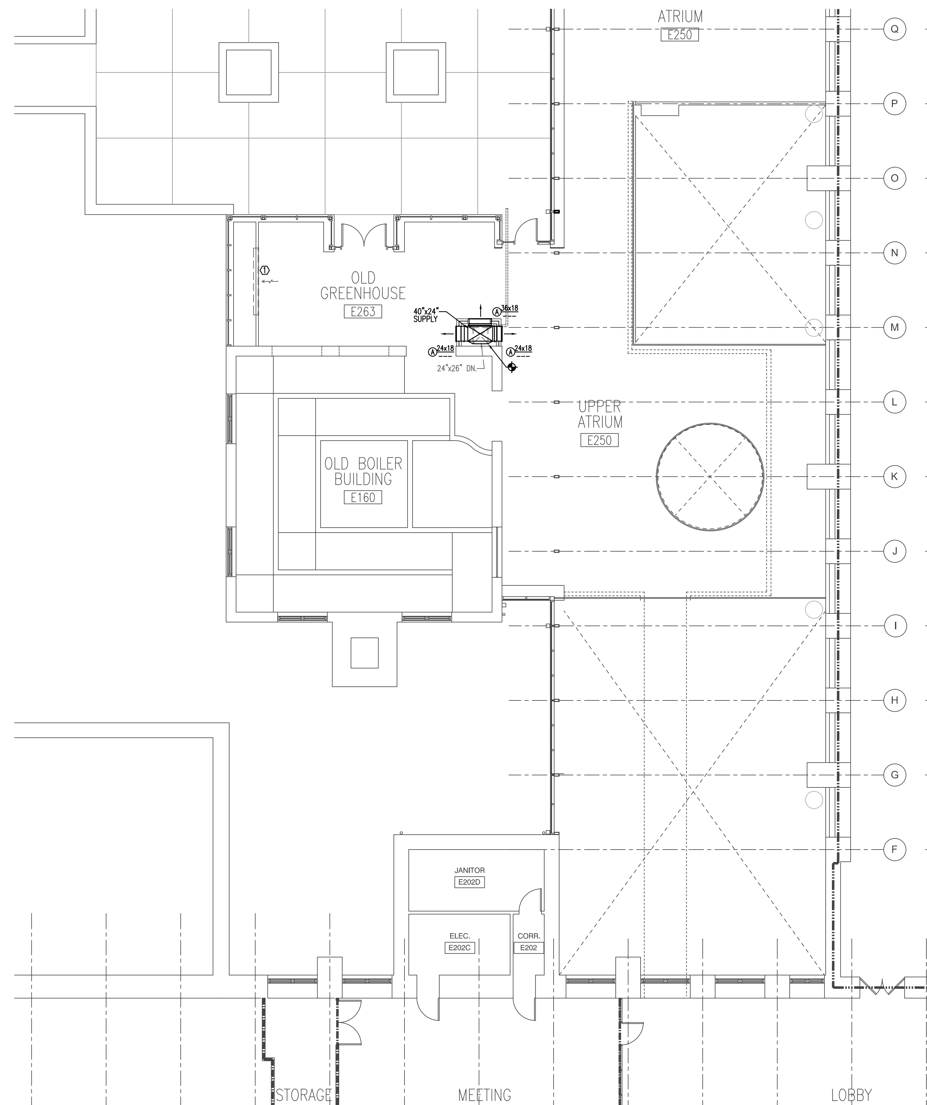
② SECOND FLOOR LEVEL - HVAC RENOVATION 1/8"=1'-0"
