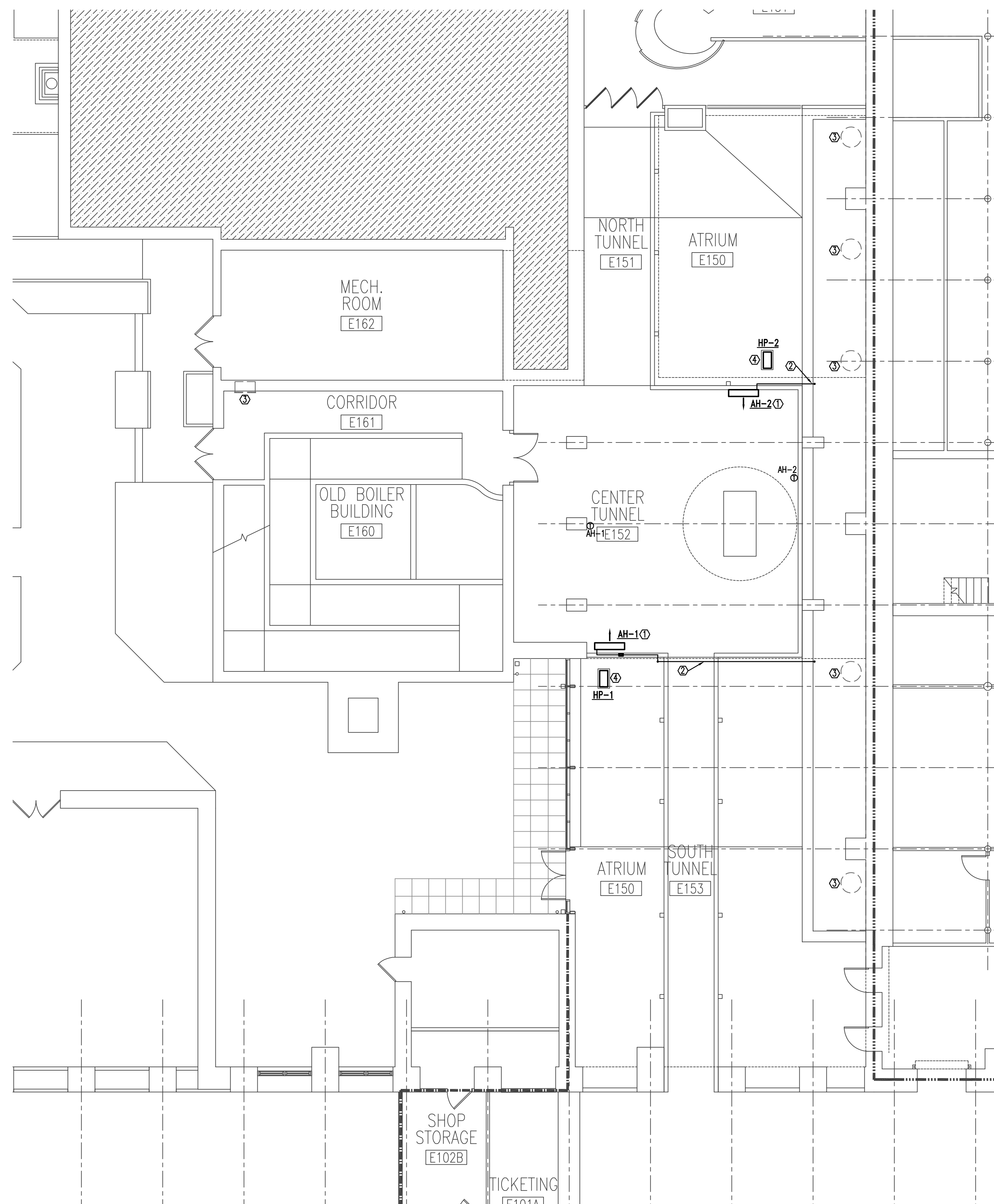
① FIRST FLOOR LEVEL - HVAC RENOVATION 1/8"=1'-0"
